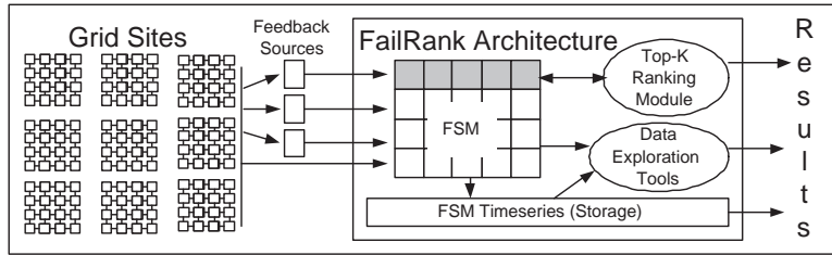
Figure 2: The FailRank System Architecture: Feedback sources are continuously coalesced into a representative array of numeric vectors, the FailShot Matrix (FSM) . FSM is then continuously ranked in order to identify the K sites with the highest potential to feature some failure.
