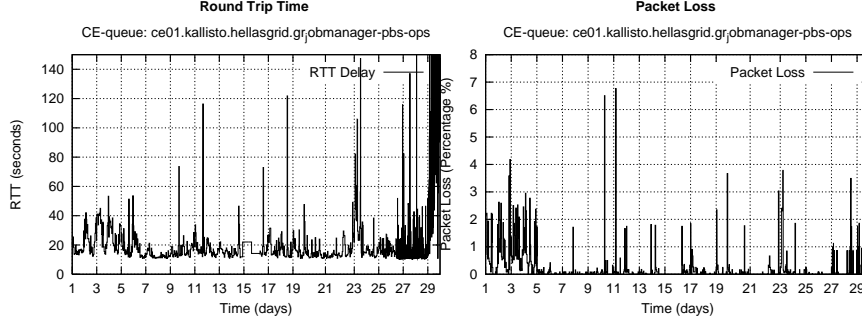
Figure 3: Round-Trip-Time (left) and Packet Loss (right) for the CE-queue ce01.kallisto.hellasgrid.gr.jobmanager-pbs-ops . These attributes are two of the 72 attributes maintained for the 2,565 CE-queues in the Failbase Repository.
