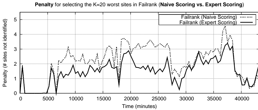
Figure 5: FailRank Scoring Function Evaluation: When the FailRank scoring function is tuned by an expert (Expert scoring) it yields more accurate results than the alternative of setting the scores uniformly (Naive Scoring).
