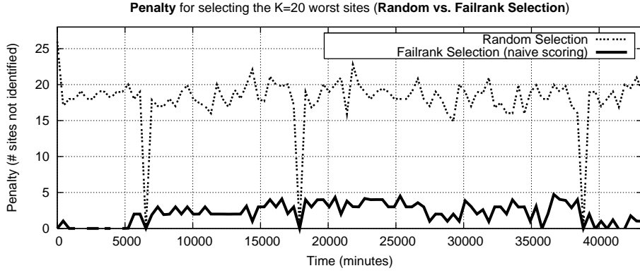
Figure 4: FailRank selection vs. Random selection: FailRank identifies the site that have failed as opposed to Random which always identifies very few of the K=20 sites.
