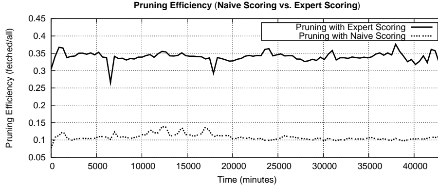
Figure 6: Pruning Efficiency: The ratio of attribute values not fetched in each time instance.
