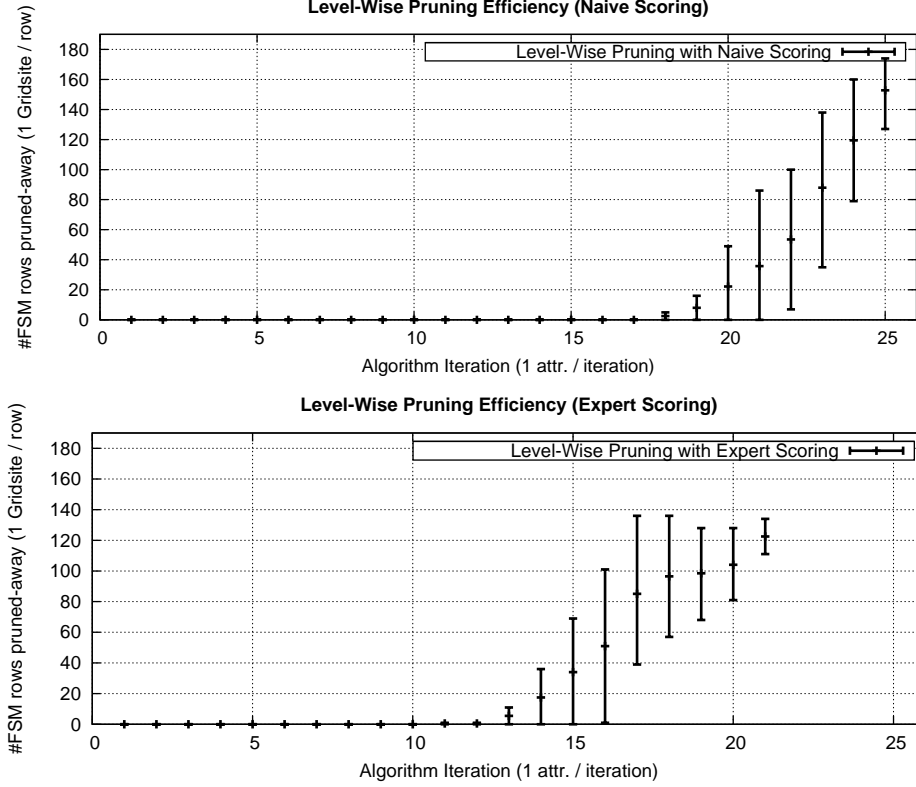
Figure 7: Level-Wise Pruning Evaluation: The number of rows excluded in each iteration of the pruning algorithm using Naive Scoring (top) and Expert Scoring (bottom).
