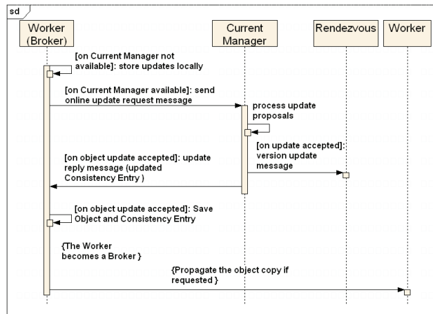
Figure 4. Update of a shared object.
