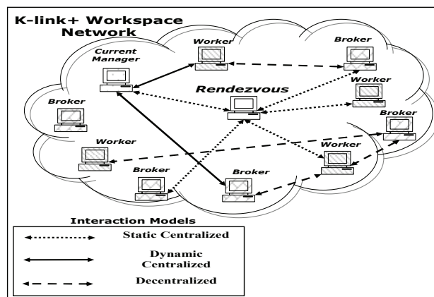
Figure 2. The K-link+ approach to content consistency. Different kinds of arrows are used to show the different models of interaction among K-link+ nodes.
