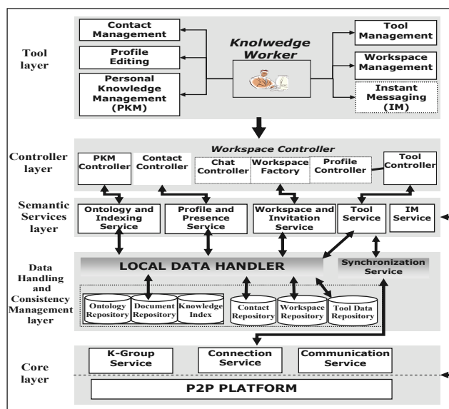
Figure 1. The K-link+ architecture.
