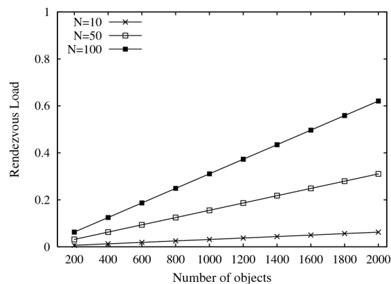
Figure 8. Load of a Rendezvous node vs. the number of shared objects, with a number of Managers equal to 6.
