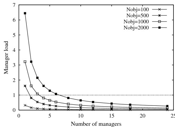
Figure 6. Manager load vs. the number of Managers, for different numbers of shared objects. The load is sustainable only when it is below the dashed line, correspond to the value of 1.
