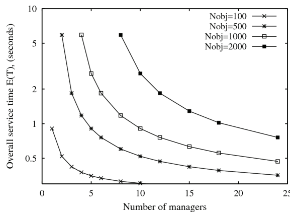
Figure 7. Overall service time of requests vs. the number of Managers, for different numbers of shared objects. When the corresponding average load is greater than 1 (see Figure 6) the service time is undefined because the system is overloaded and the requests cannot be served.
