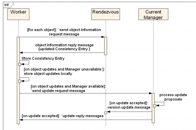
Figure 5. Peer synchronization.
