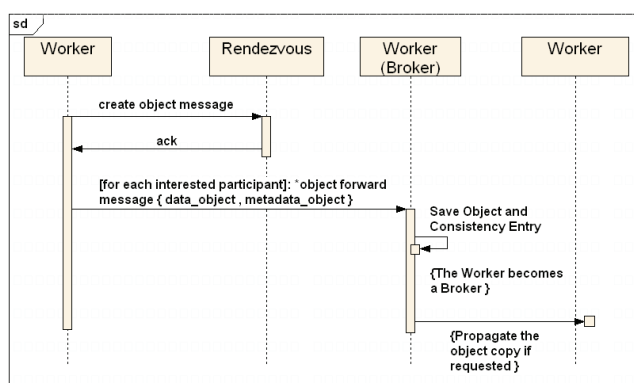
Figure 3. Creation of a new shared object.
