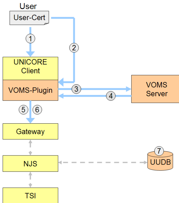
Figure 3: Architecture of the UNICORE and VOMS integration
