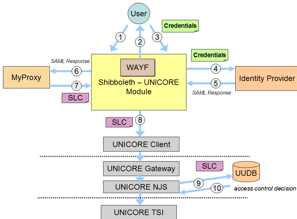
Figure 4: Integration of UNICORE and Shibboleth
