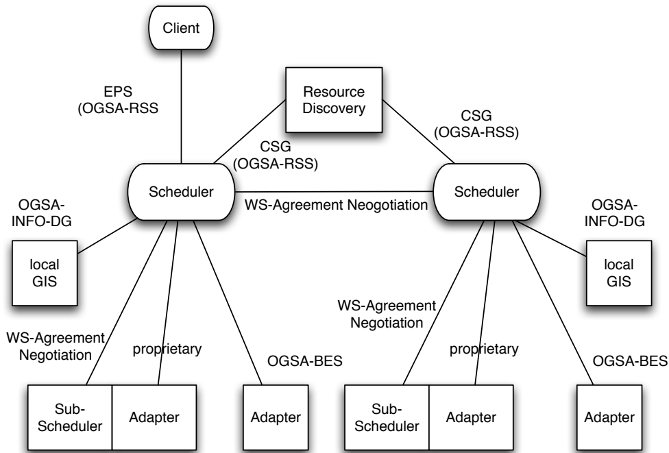
Figure 1: Grid Scheduler interoperation including OGSA components
