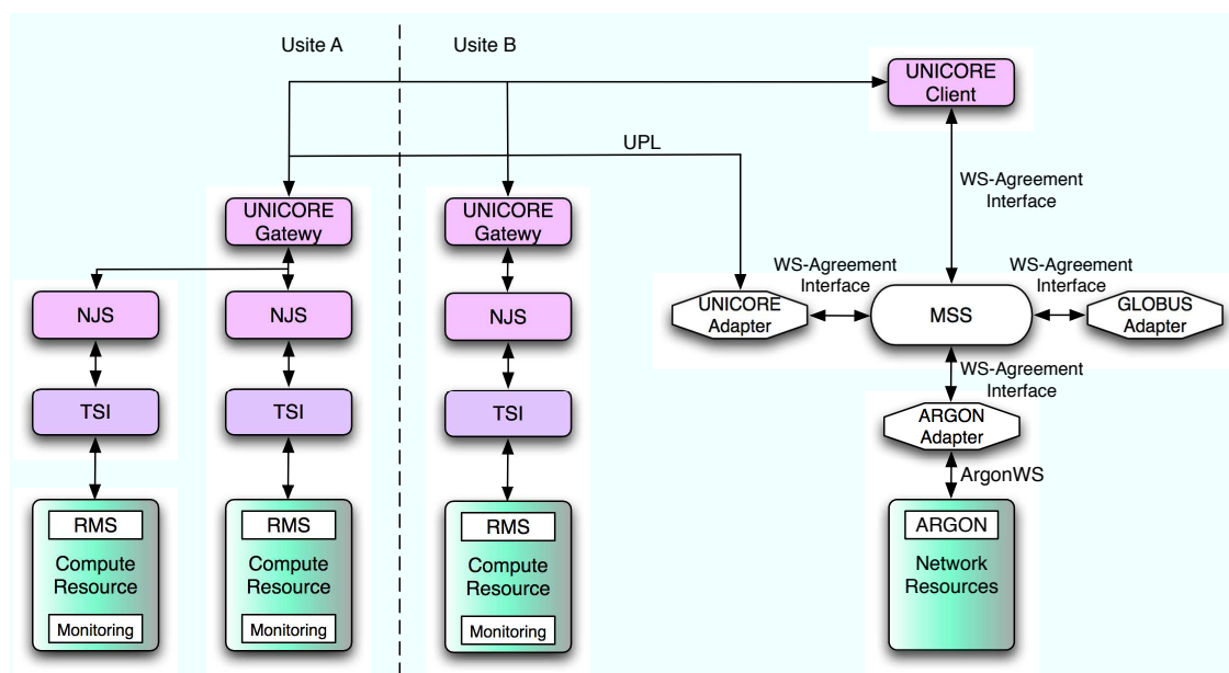
Figure 3: Architecture of the MetaScheduling Environment
