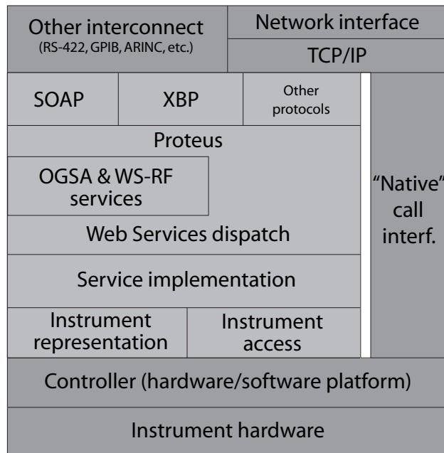
Figure 1: Common Instrument Middleware Architecture (CIMA) [6]
