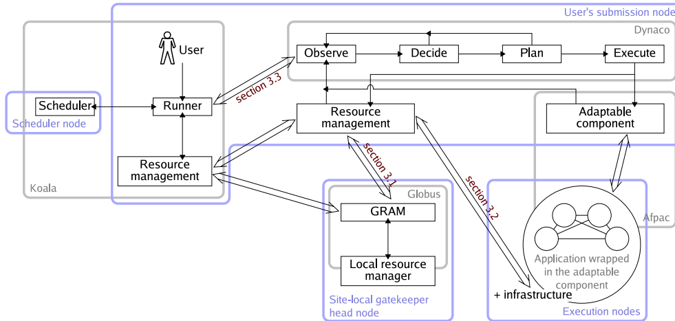
Figure 1: Overall architecture of an adaptable application that uses DYNACO and that is deployed into a grid operated by KOALA and GLOBUS. Single arrows show the bindings between elements within each design pattern. Double arrows connect elements that interface design patterns together.
